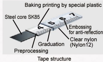
Tape structure
