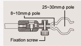
▶ FLEXIBLE SYSTEM (FPPS2)
