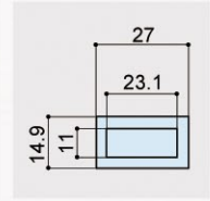
Dimensions (MTR-22)
